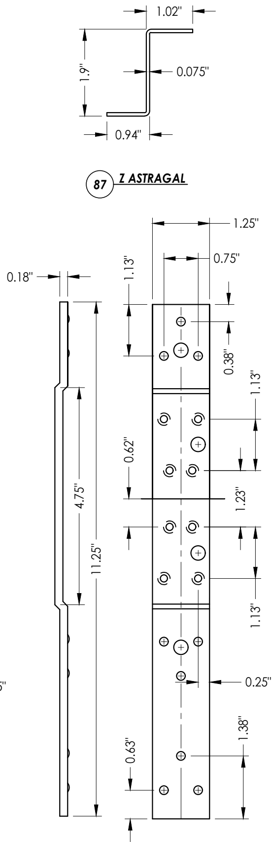
22 STANDARD (LONG) DOOR HINGE Reinforcement top hinge
